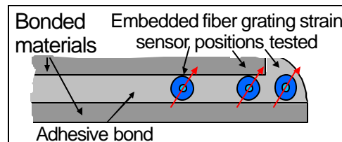
Figure 2. Multi-axis Strain Sensors Embedded into Inner (left) and Edge (middle), and Retro-fitted (right), Locations of Adhesive Bond
