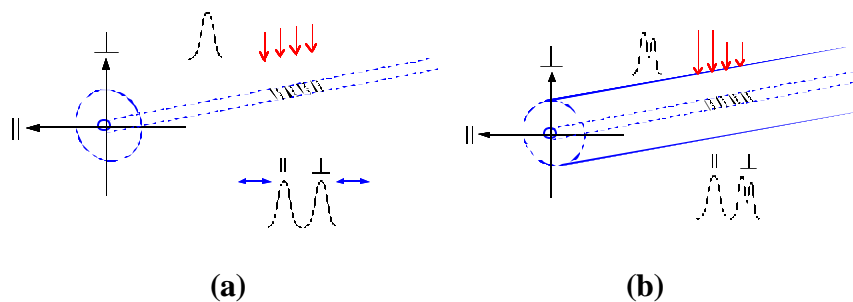
Figure 1. The Effect of Strain on a Multi-Axis Fiber Grating
