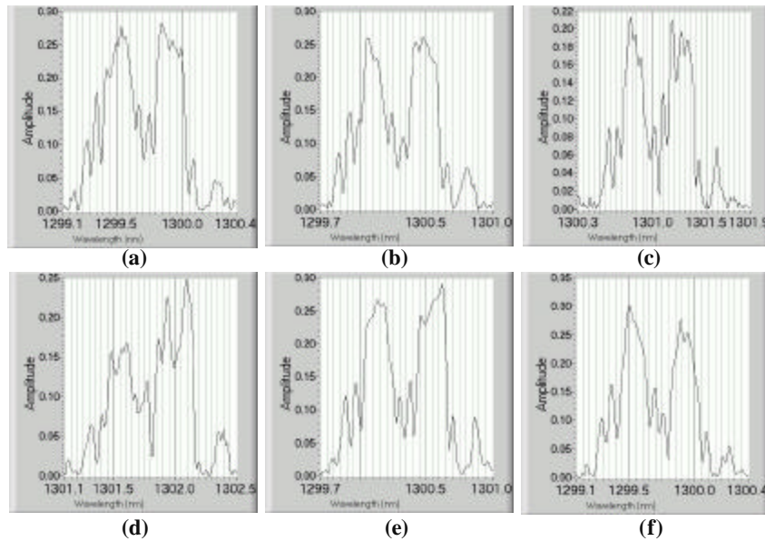
Figure 8. Spectral Profiles from Sensor 8, Third Pressure Cycle Dual-axis fiber grating sensor approximately 2.5 cm from the cut tow damage site during the third pressure (a) 0 psi, (b) 333 psi, (c) 666 psi, (d) 1000 psi (e) 333 psi return and (f) 0 psi return.
