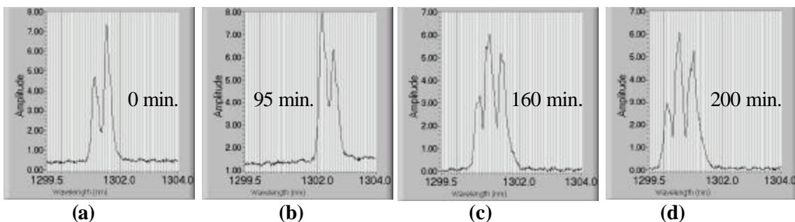
Figure 4. Sensor 2 was monitored during the cure cycle. (a), (b) Increasing temperature to peak temperature; (c), (d) cool down.
