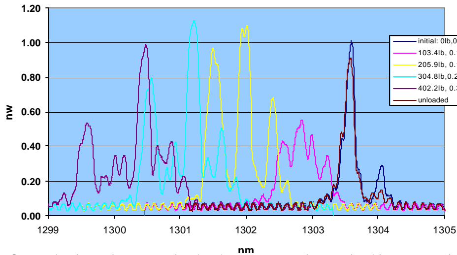
Figure 8. Dual axis grating sensor in glass/epoxy composites strained in compression, left peak
